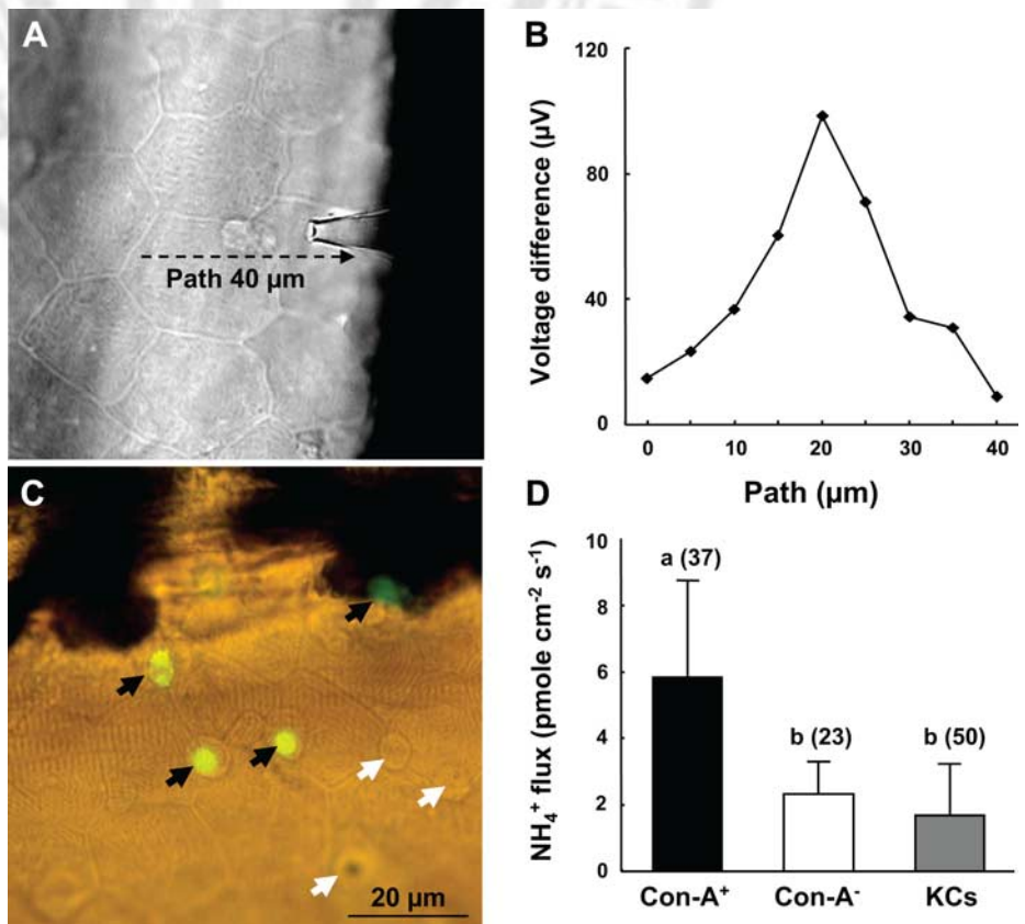
Fig. 2. NH 4 + fluxes at H + pump-rich cells (HRCs) [concanavalin A + (Con-A + )], keratinocytes (KCs), and other ionocytes (Con-A - ). A: under a microscope, apical membranes of ionocytes were identified, and a “line scan” was made by probing at a series of locations along a line (arrow) across the surface of the ionocytes and adjacent keratinocytes. B: measured NH 4 + fluxes of the line scan over the surface of an HRC are shown. C: the measured ionocytes were further discriminated into a Con-A + (HRC) or Con-A - (non-HRC) group by fluorescent Con-A labeling. D: NH 4 + effluxes (means ± SD, n = 37, 23, and 50, respectively) from different types of cells were compared. Different letters indicate a significant difference (one-way ANOVA, P < 0.05).
