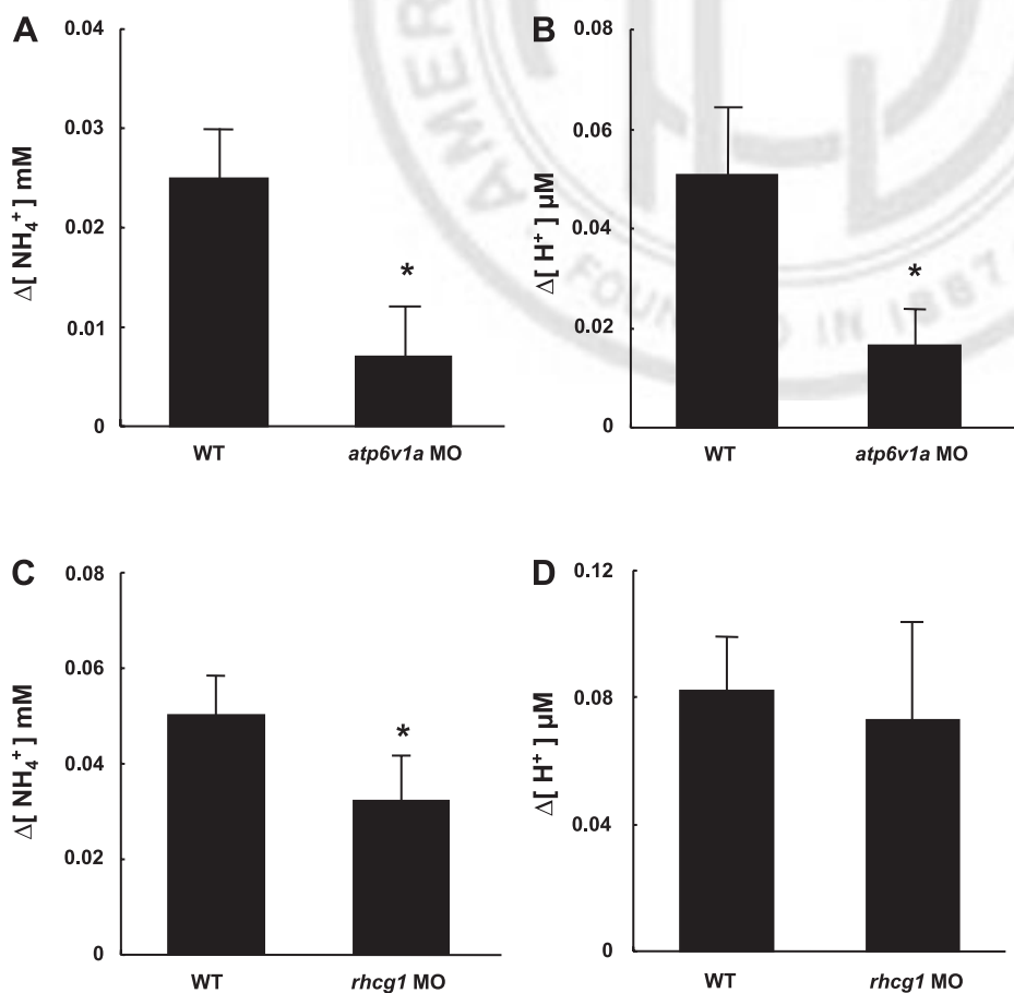
Fig. 6. \Delta[\text{NH}_4^+] (A and C) and \Delta[\text{H}^+] (B and D) at the yolk sac surface of wild-type (WT) larvae and morpholino (MO)-injected larvae. The morpholino against atp6v1 or rhcgl was injected at the 1- to 4-cell stage of larvae, and the larvae were measured at 5 dpf. Different batches of embryos were used for the atp6v or rhcgl injection. Data are presented as means \pm SD ( n = 10 ). *Significant difference (Student's t -test, P < 0.05 ).
